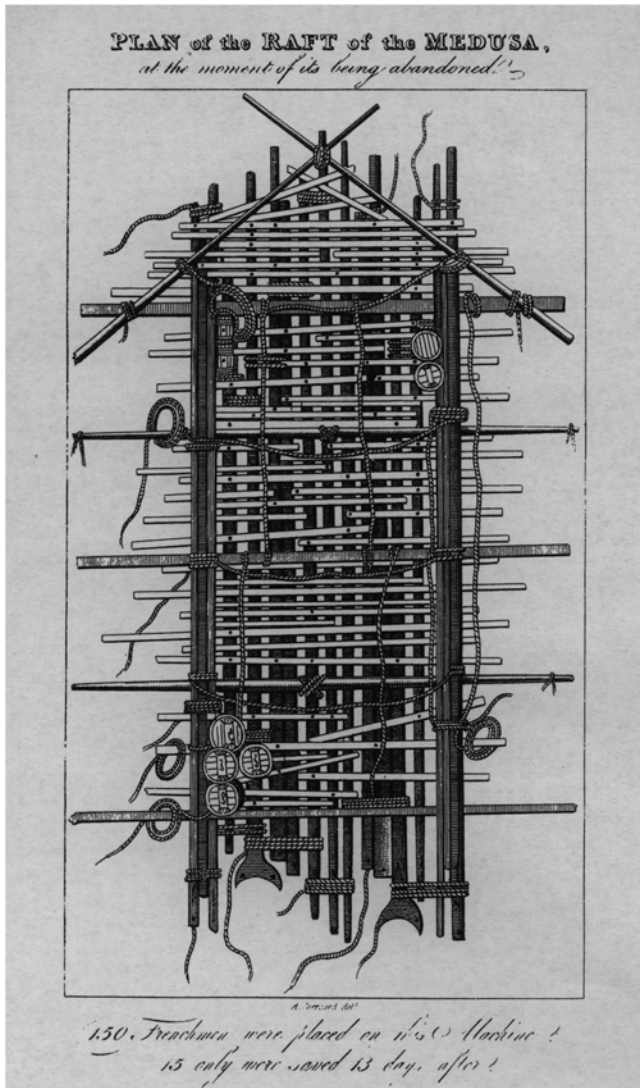
Abb. 4 Das von den Überlebenden improvisiert zusammengebaute Floß der LA MÉDUSE (1816). (Aus: Alexander Correard, J.B. Henry Savigny: Narrative of a Voyage to Senegal in 1816. Undertaken by Order of the French Government, Comprising an Account of the Shipwreck of the MEDUSA, the Suffering of the Crew, and the Various Occurrences on Board the Raft, in the Desert of Zaara, at St. Louis, and at the Camp of Daccard, to which are Subjoined Observations Respecting the Agriculture of the Western Coast of Africa, from Cape Blanco to the Mouth of the Gambia. Nachdruck London 1968, gegenüber S. 1)
